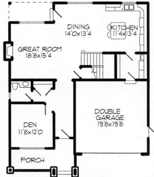
MAIN FLOOR PLAN 1062 SQ.FT.
