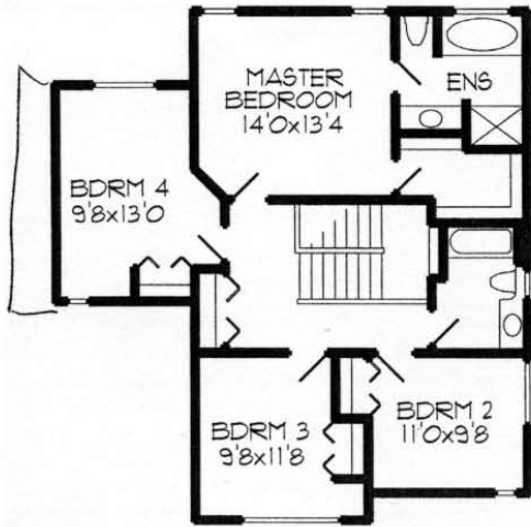
SECOND FLOOR PLAN 964 SQ.FT. 2026 TOTAL SQ.FT.
