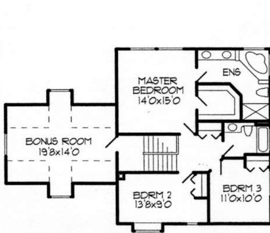
SECOND FLOOR PLAN 824 SQ.FT. + BONUS ROOM 316 SQ.FT. + 1140 TOTAL
