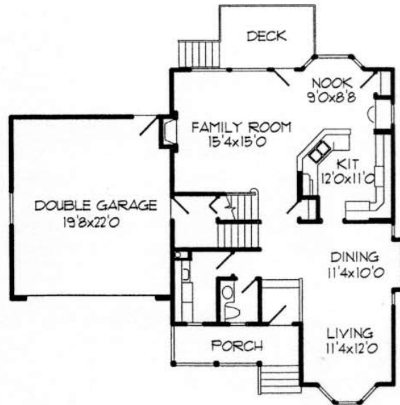
MAIN FLOOR PLAN 1020 SQ.FT. 2160 TOTAL SQ.FT.
