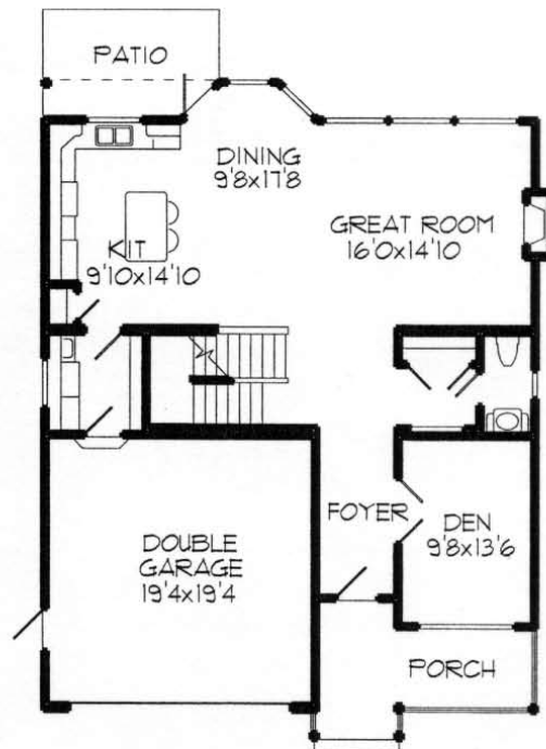
MAIN FLOOR PLAN 1066 SQ.FT.
