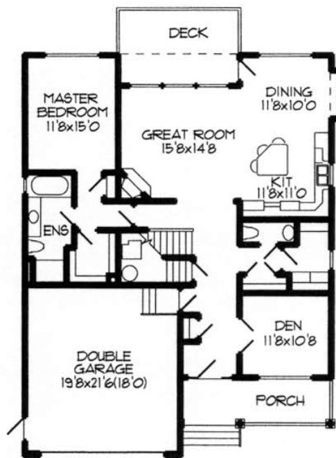
MAIN FLOOR PLAN 1396 SQ.FT.
