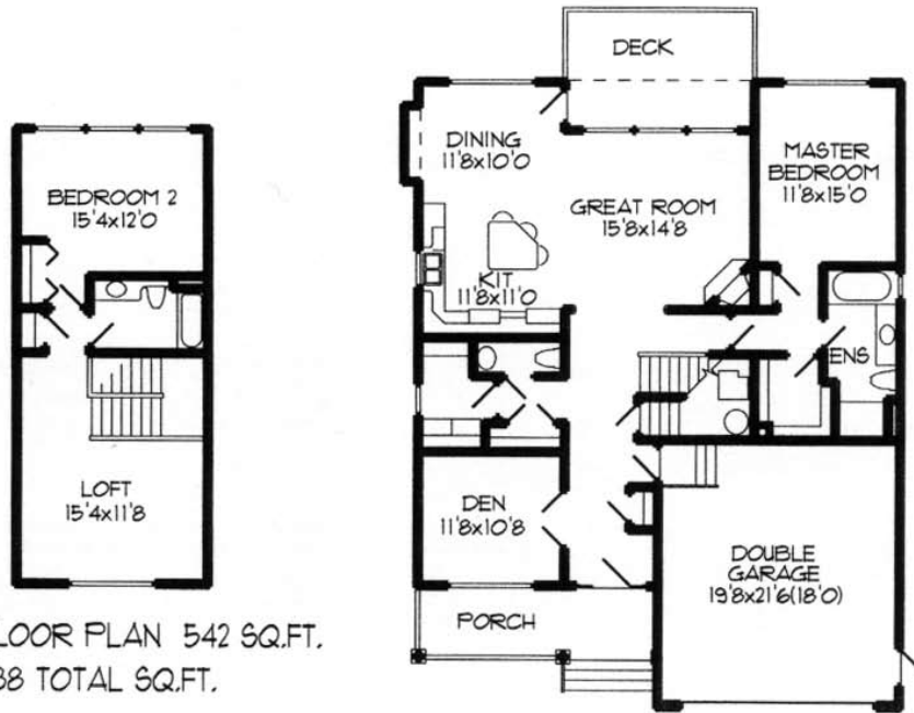
MAIN FLOOR PLAN 1396 SQ.FT.
